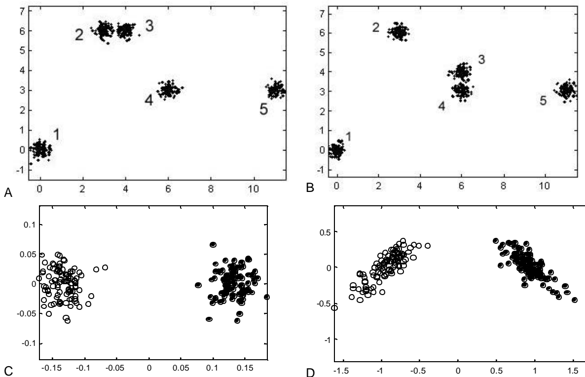
Figure 3. Results from a sampling experiment comparing PCA ordinations based on Procrustes alignments and those based on interlandmark distances. A and B show isotropic scatter around five landmarks for 100 specimens. C The results of a principal components analysis using projections of Procrustes aligned specimens in the tangent space (equivalent to using partial warp scores and the uniform component). As expected, two distinct circular scatters are shown because the two populations differ only in mean shape. D The results of a principal components analysis using Rao & Suryawanshi (1996) shape variables. Note the different pattern of strong covariances within each group. The effect is more extreme than shown in Figure 9
